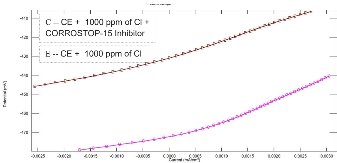
Fig.12 Linear polarization behaviour of steel rebar in systems {CE + 1,000 ppm of Cl} and {CE + In + 1,000 ppm of Cl}
