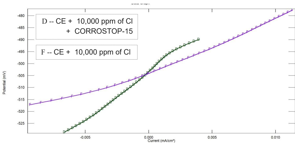
Fig.13 Linear polarization behaviour of steel rebar in systems {CE + 10,000 ppm of Cl} and {CE + In + 10,000 ppm of Cl}
